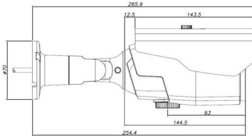
DIMENSION
