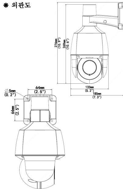
TR-JB07-D-IN
